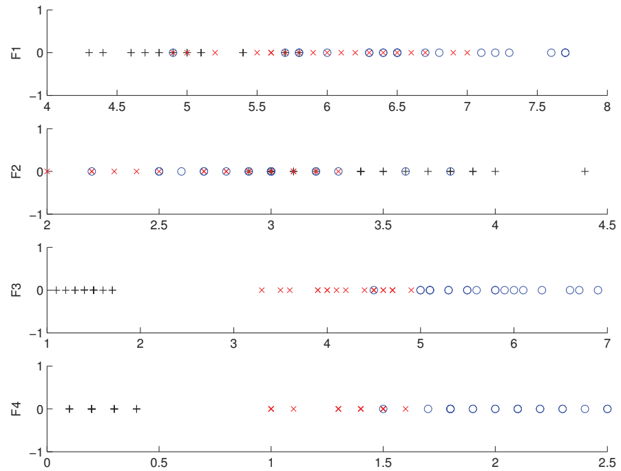
Figure 6.1 Plot of the training data for single features on Iris dataset; the three classes are shown with different symbols. It can be seen that F4 by itself allows quite good discrimination.
